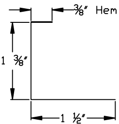
Single Wall Ring Profile
