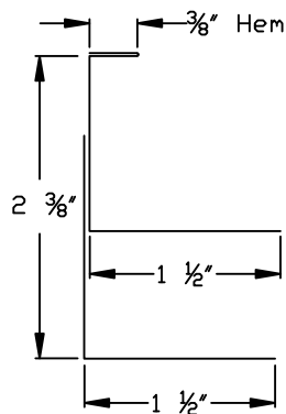
1" Double Wall Ring Profile
