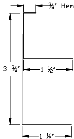
2" Double Wall Ring Profile
