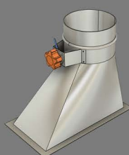
STO Sticky W/ Damper & Bracket Stand-off w 3/8"Continuous Rod
